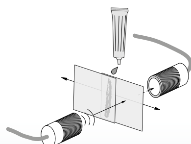
Ultrasonic splice monitoring
